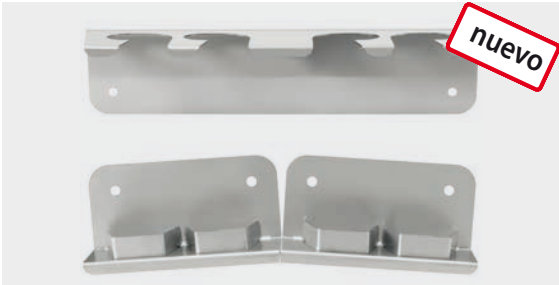
For all lances with R + M / Suttner insulation. With 4 lance fixations for mounting for connection: hand screw coupling or female thread
