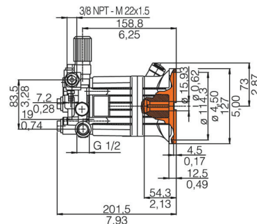
Electric Flange AXD/S-E
