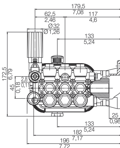
Electric Flange BWD-E
