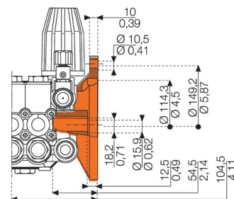
Electric Flange LW-K E
