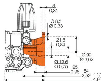
Gas Flange LW-K G
