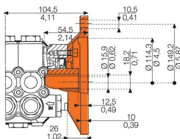
Electric Flange LW-E
