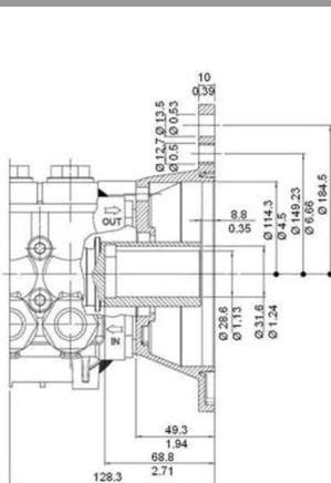
Gas Flange FW2-G
